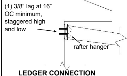
LEDGER CONNECTION
